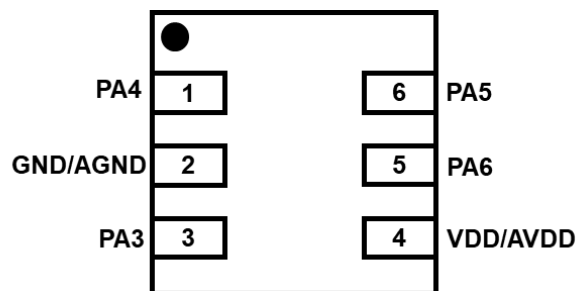
PMS161-2N06: DFN6 (2*2mm)
