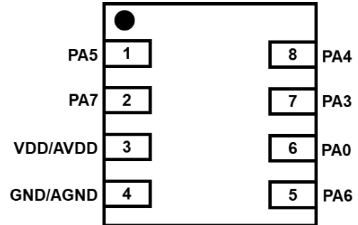
PMS161-2N08B: DFN8 (2*2mm)
