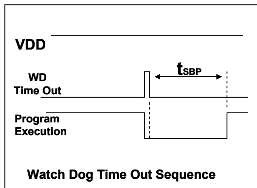
Fig. 10: Sequence of Watch Dog Time Out
