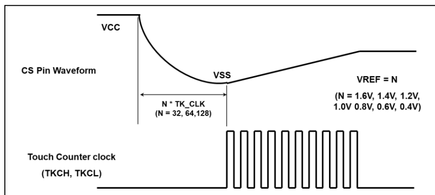
Fig. 18: Timing diagram of Touch converting progress
