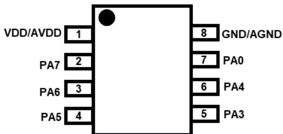
PMS161-S08A: SOP8 (150mil)
