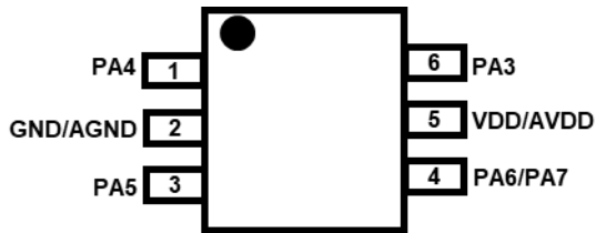
PMS161-U06A: SOT23-6 (60mil)
