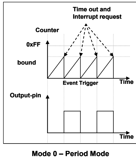
Mode 0 – Period Mode Fig. 14: Timing diagram of Timer2 in period mode
