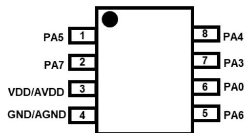
PMS161-S08B: SOP8 (150mil)
