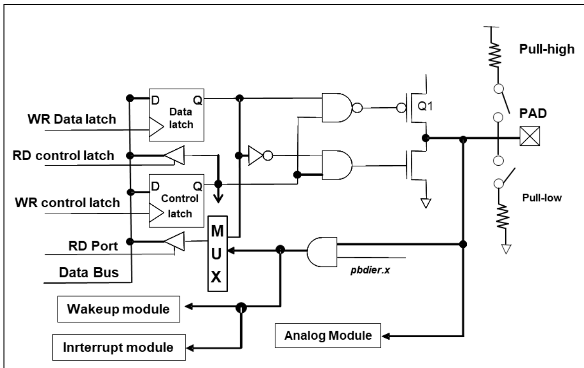
Fig. 12: Hardware diagram of IO buffer
