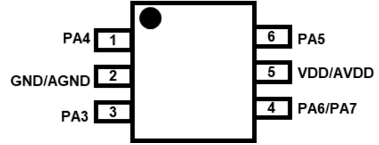
PMS161-U06B: SOT23-6 (60mil)
