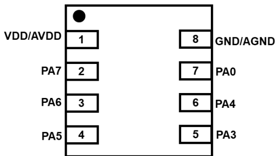
PMS161-2N08A: DFN8 (2*2mm)
